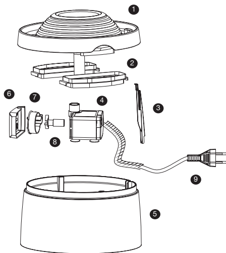
1. Water bowl | 2. Carbon filter | 3. Stain relief | 4. Pump head | 5. Water reservoir | 6. Pump cover | 7. Impeller cover | 8. Impeller | 9. Power cord
