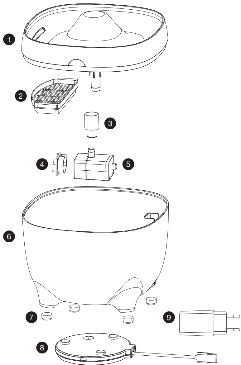
1. Waterdispenser | 2. Filter holder | 3. Water outlet pipe | 4. Pump cover | 5. Wireless water pump | 6. Water tank | 7. Anti slip feet | 8. Power base | 9. USB Power adapter
